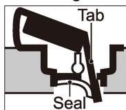
Valve diagram
